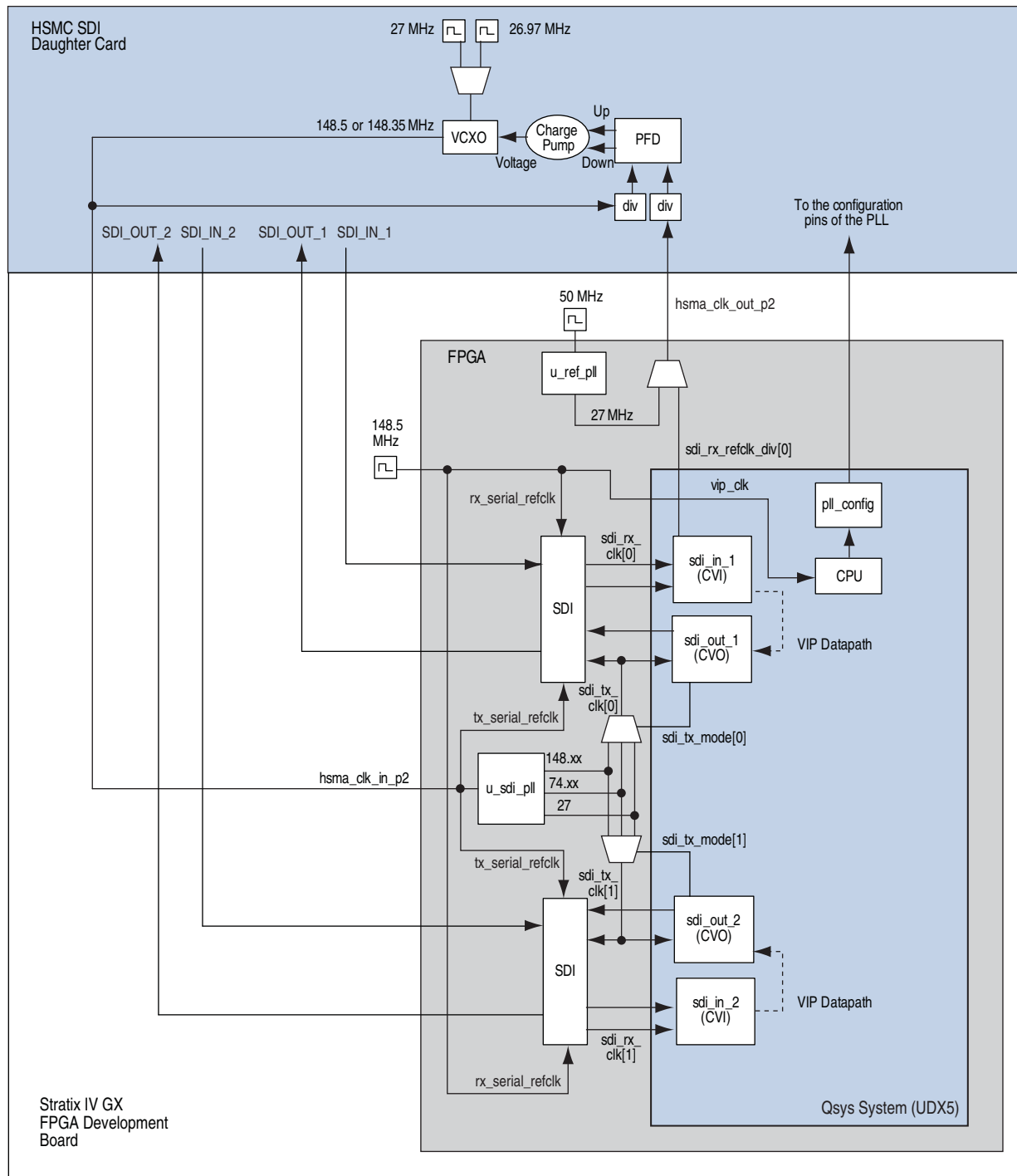
Figure 3. Top-Level Clock Connections for SDI Data and Control
