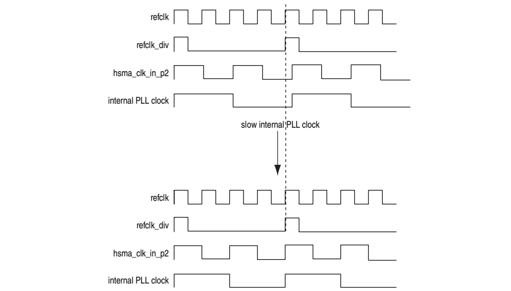
Figure 4. Clock Locking
