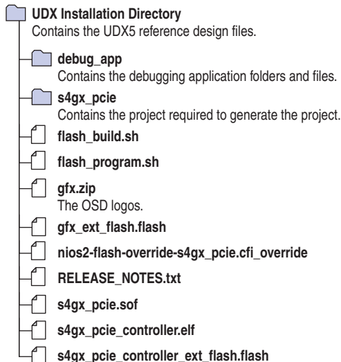
Figure 10. Reference Design Directory Structure
