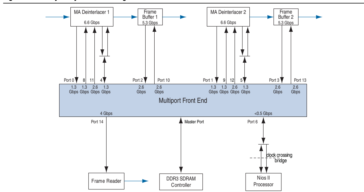
Figure 6. Memory Subsystem Block Diagram
