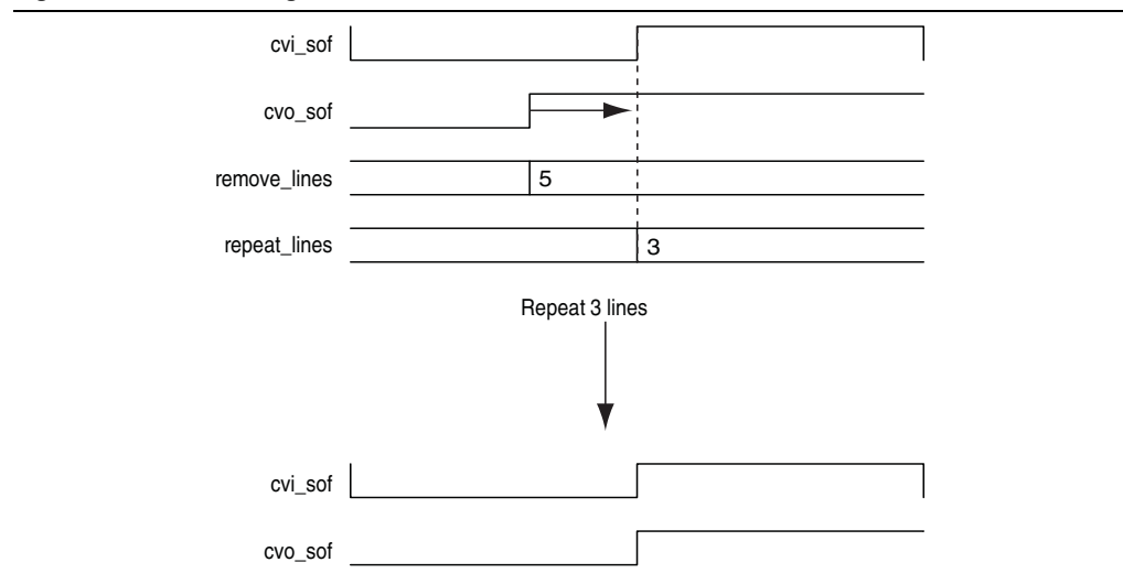
Figure 5. Frame Locking
