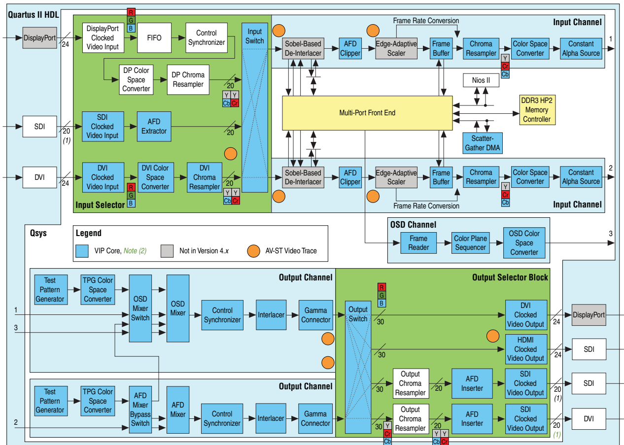
Figure 2. UDX5 Reference Design Block Diagram
