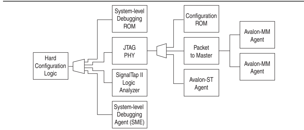
Figure 9. Debugging System on the Board
