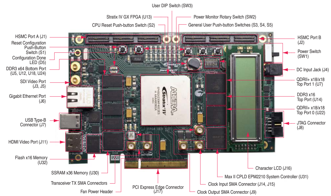
Figure 1. Stratix IV GX FPGA Development Board
