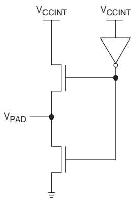
Figure 7. ESD Protection Circuitry in CPLD Devices
