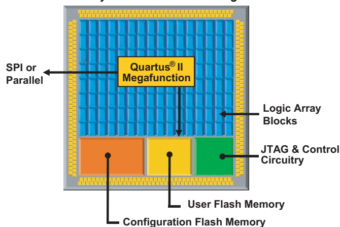
Figure 1. User Flash Memory Interface to Core Logic & JTAG
