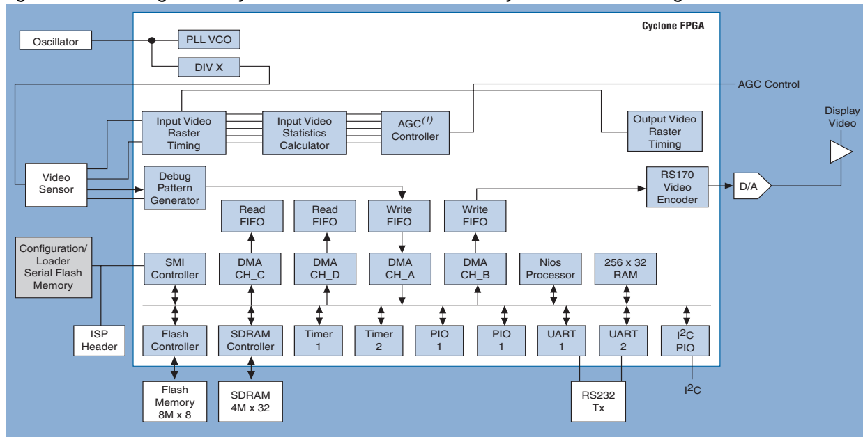
Figure 1. Block Diagram of Cyclone Series FPGA Functionality Within Intevac’s NightVista Camera
