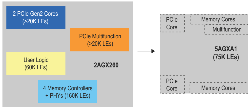
Figure 5. Hard IP Blocks Reduce FPGA User Logic Requirements and Lower Implementation Costs
