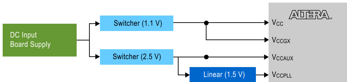
Figure 6. Arria V FPGAs Require the Fewest Number Power Rails of Any Midrange FPGA
