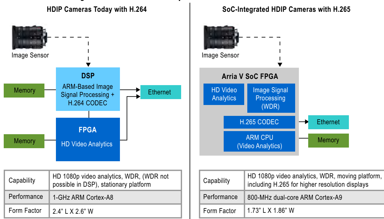
Figure 10. HD IP Camera Developmental Evolution
