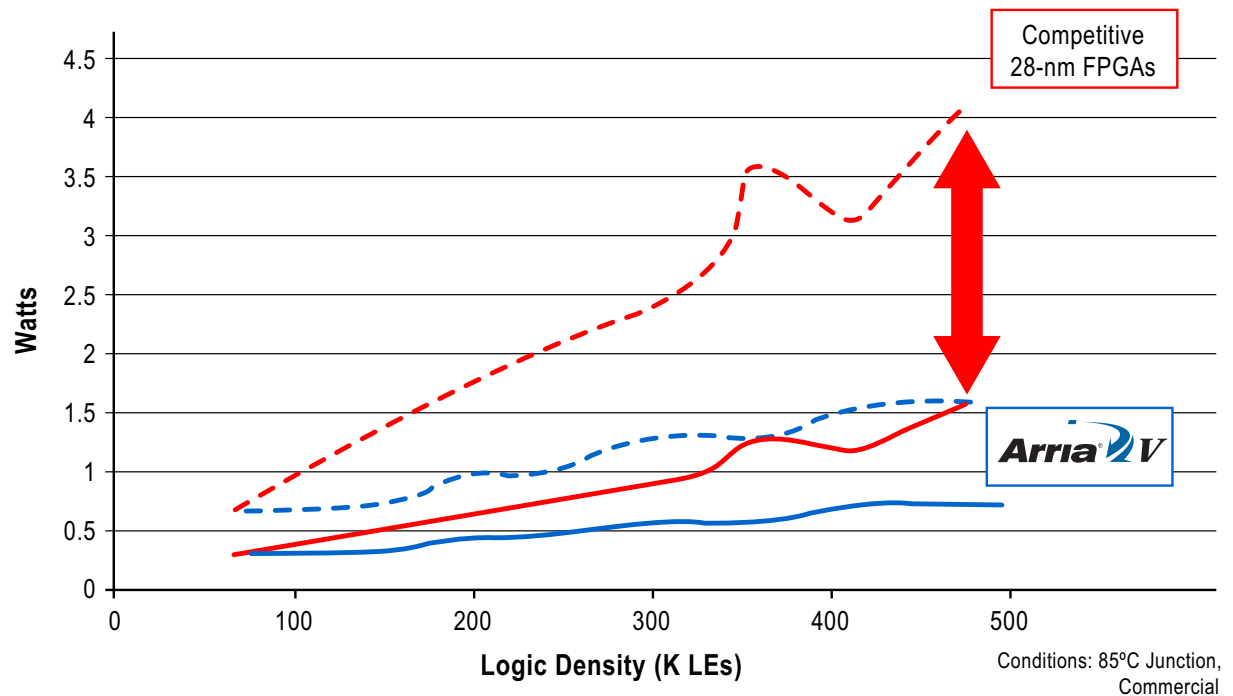
Figure 8. Static Power Consumption of Arria V FPGAs Compared to Other 28-nm Midrange FPGAs
