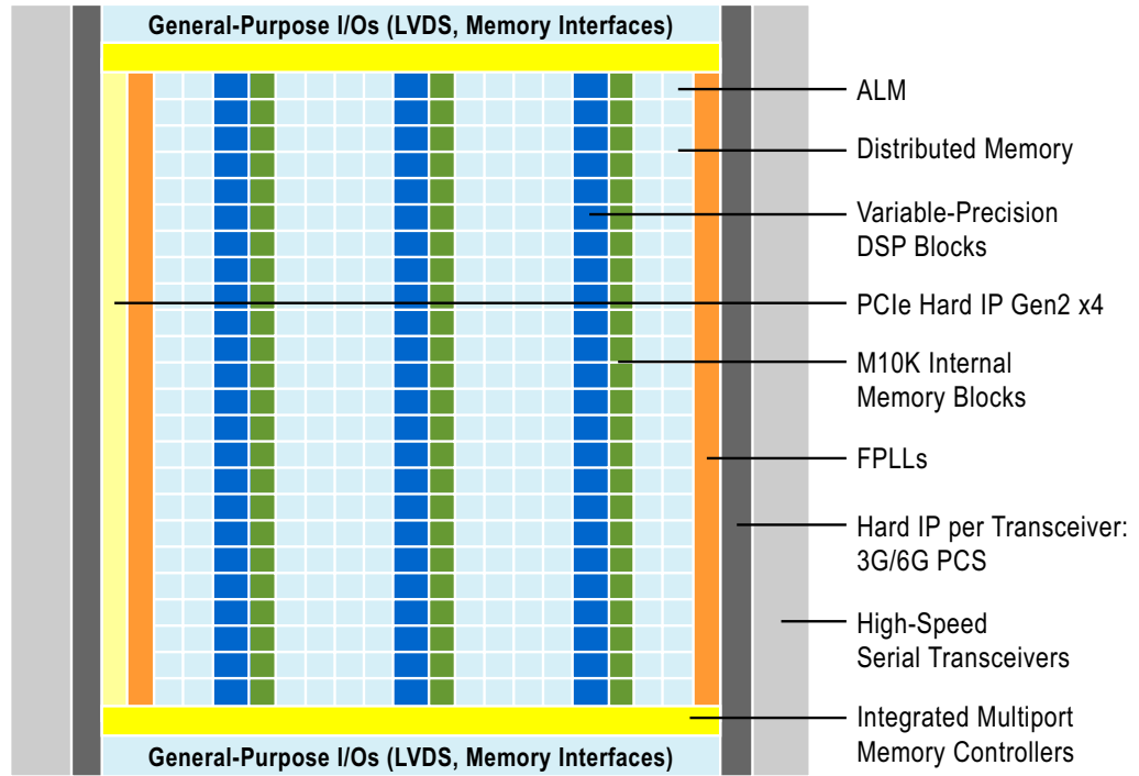
Figure 1. Block diagram of Arria V FPGA
