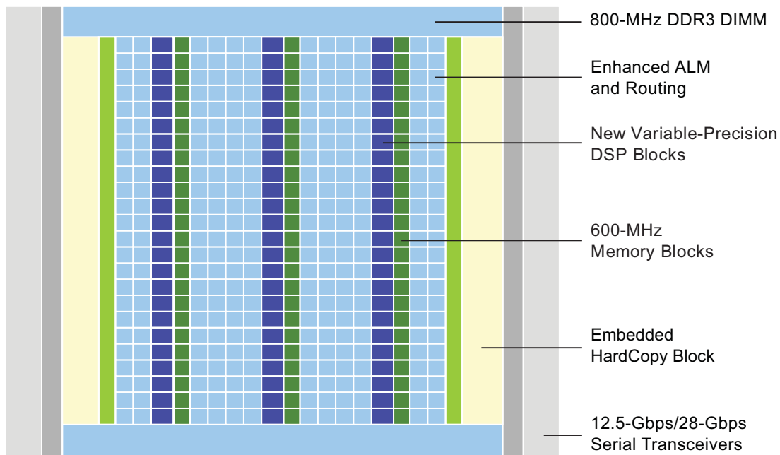
Figure 8. Stratix V FPGA I/O and Fabric Functional Blocks Enabling Higher System Performance
