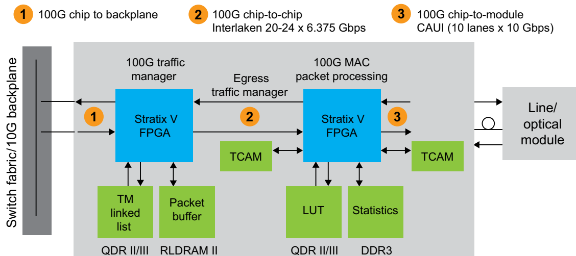
Figure 7. 100-GbE Line Card Using Two Stratix V FPGAs
