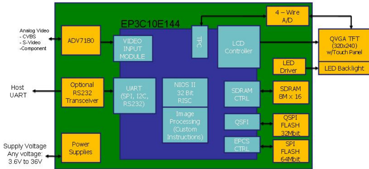
Figure 2. Thomas II Design Block Diagram
