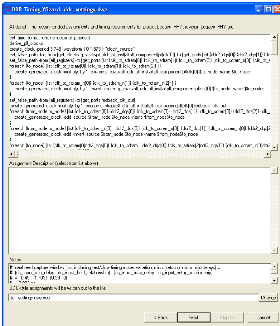
Figure 2–7. Timing Assignments to be Added to the Project
