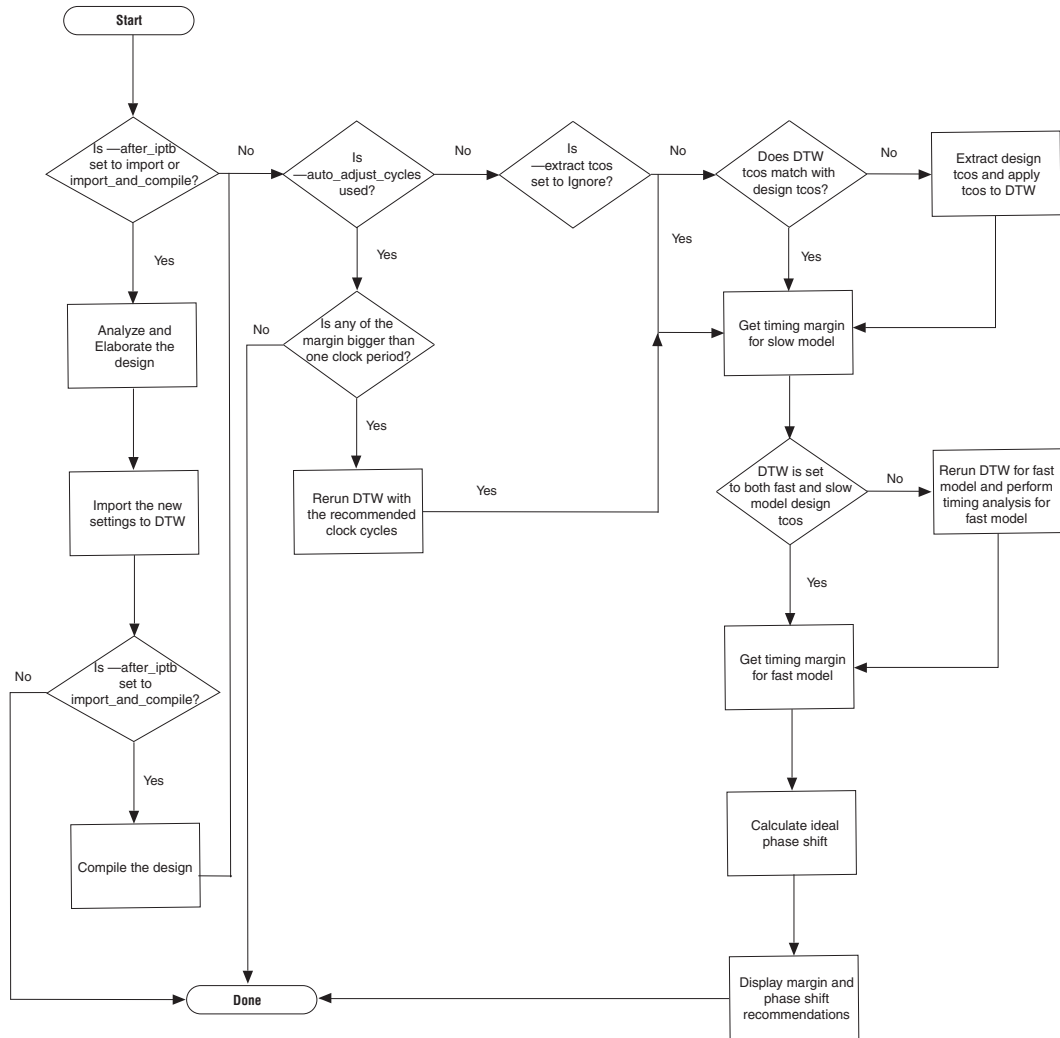
Figure 3-1. The dtw_timing_analysis.tcl algorithm
