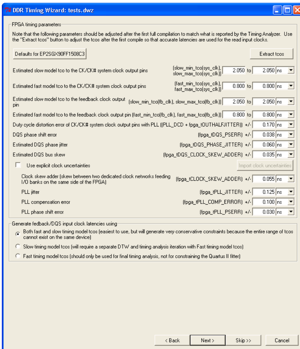
Figure 2–27. FPGA Timing Parameters Page When Using Classic Timing Analyzer Names
