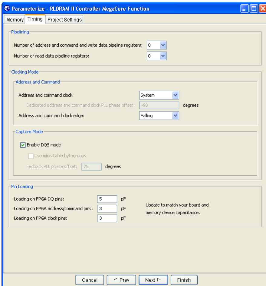
Figure 3-7. RLDRAM II MegaWizard Timing Panel
