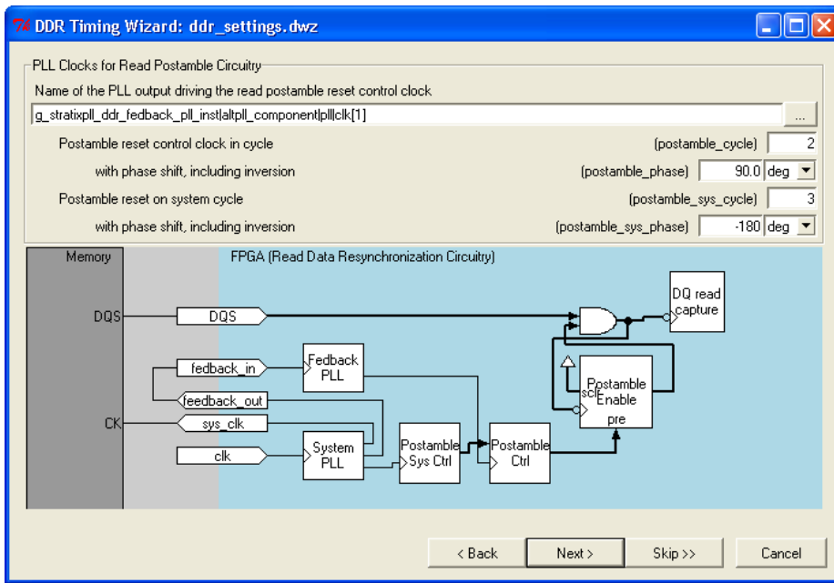
Figure 2–22. Postamble Clock Connectivity
