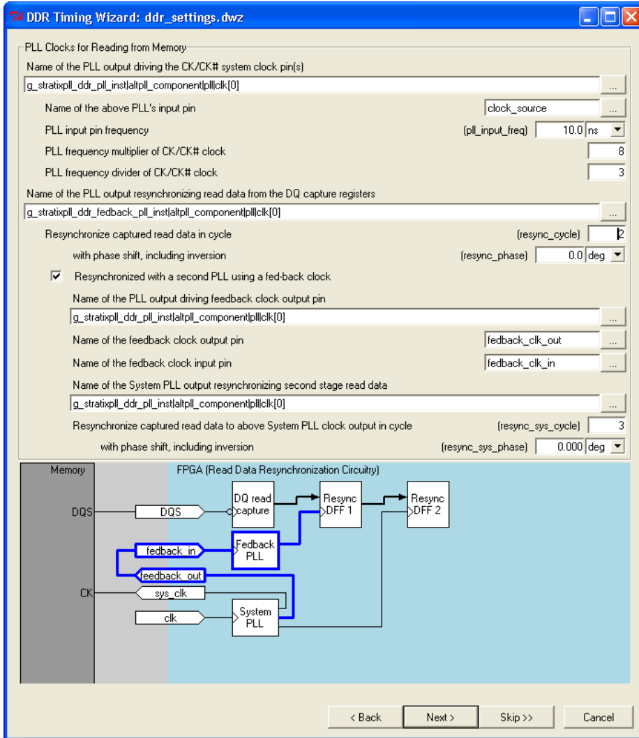
Figure 2–20. Feedback Resynchronization Path (Highlighted)
