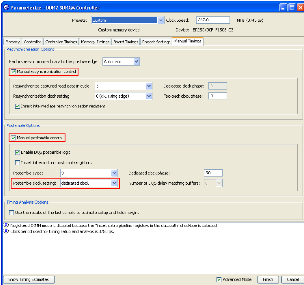
Figure 3–8. Initial Resynchronization, Postamble Clock Cycle, and Phase Shift Selections
