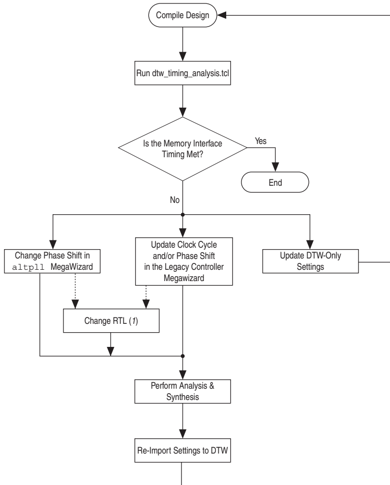
Figure 3–6. Timing Closure Process
