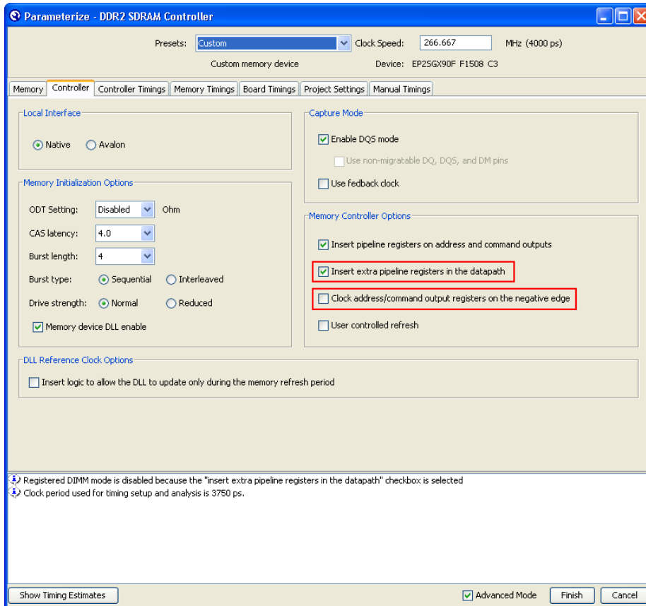
Figure 3–15. Preparing for Dedicated Address/Command Clock
