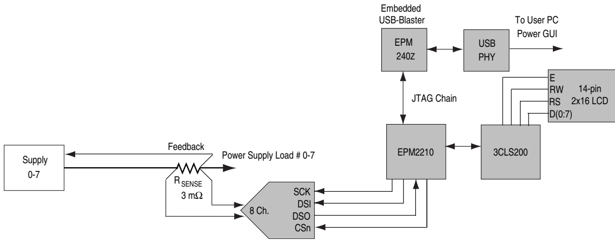
Figure 2-11. Power Measurement Circuit
