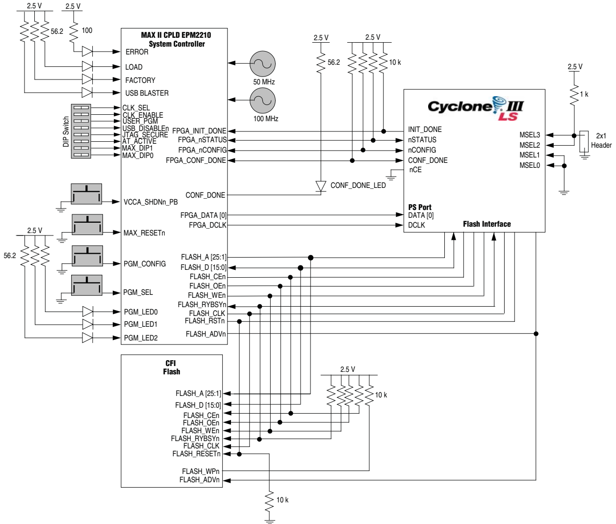
Figure 2-5. PFL Configuration
