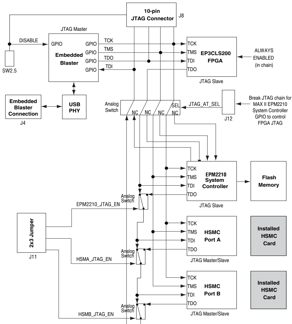
Figure 2-4. JTAG Chain
