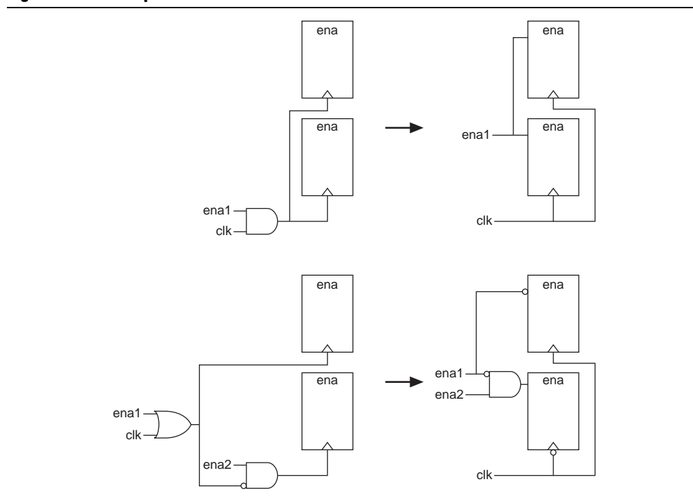
Figure 14-3. Example Gated Clock Conversion
