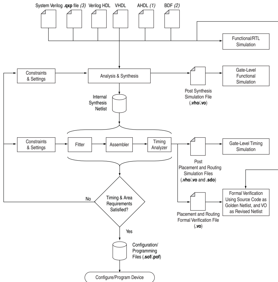
Figure 14-1. Quartus II Design Flow Using Quartus II Integrated Synthesis
