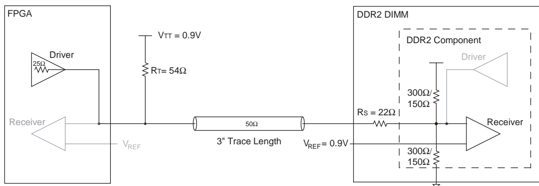
Figure 5-4. Double Parallel Termination Scheme (Class II) Using ODT on DDR2 SDRAM DIMM with Memory-Side Series Resistor
