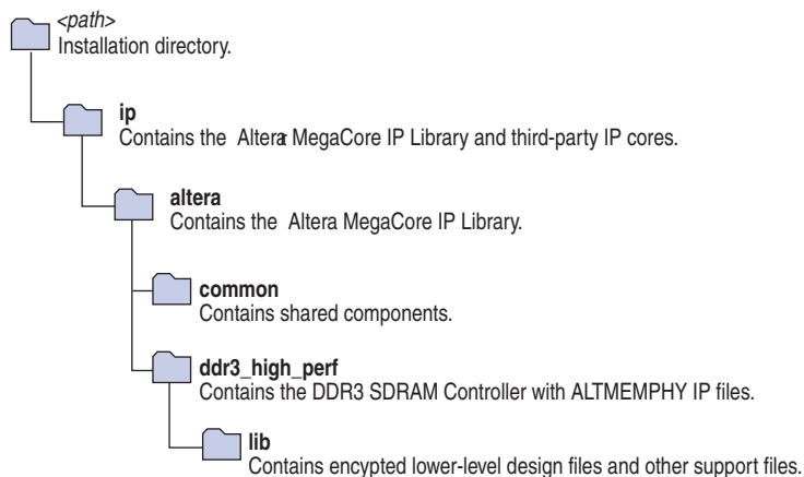
Figure 13-2. Directory Structure
