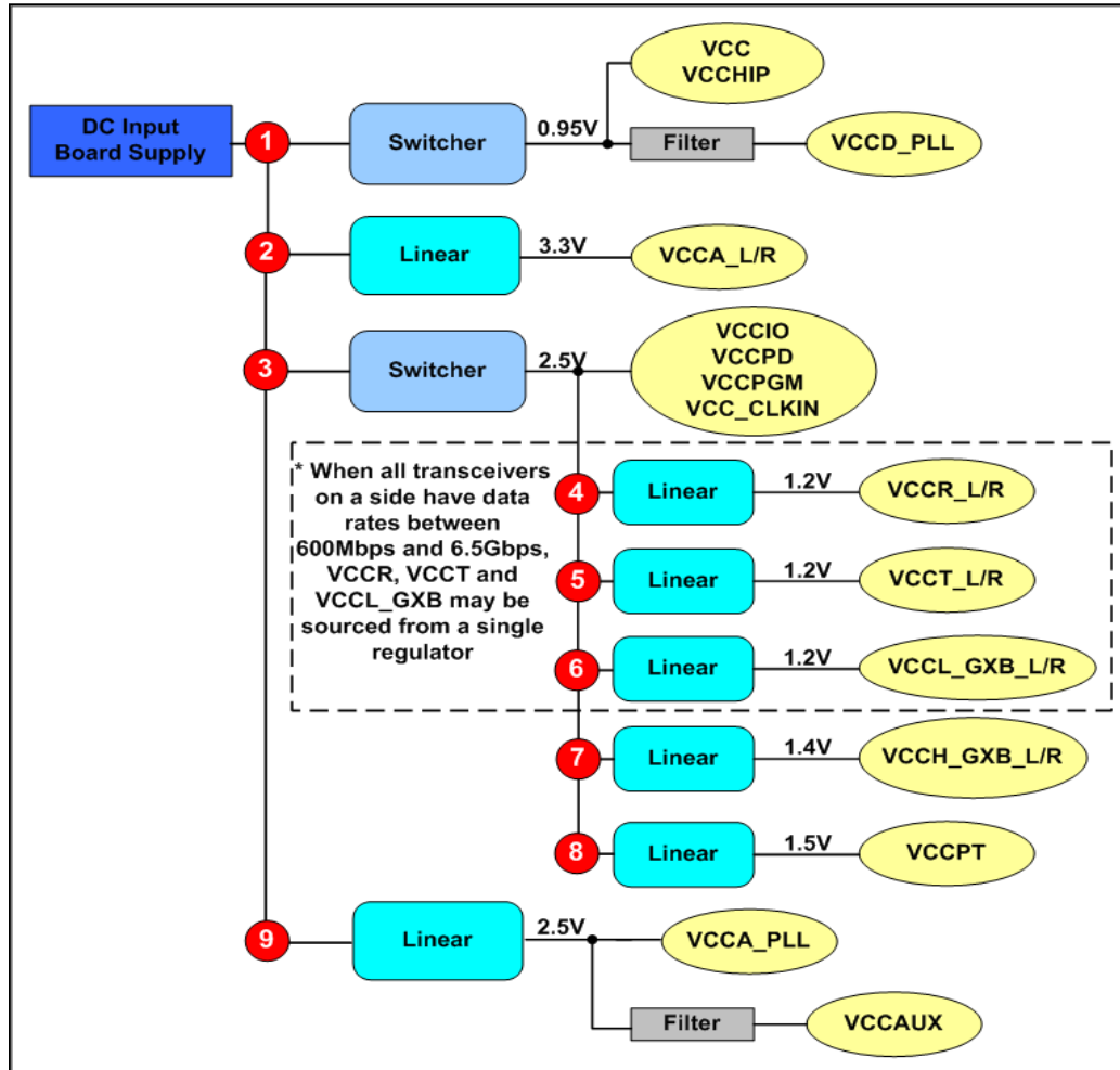
Figure 1. Example Stratix IV GT Power Supplies Block Diagram for Data Rates > 2.488 Gbps
