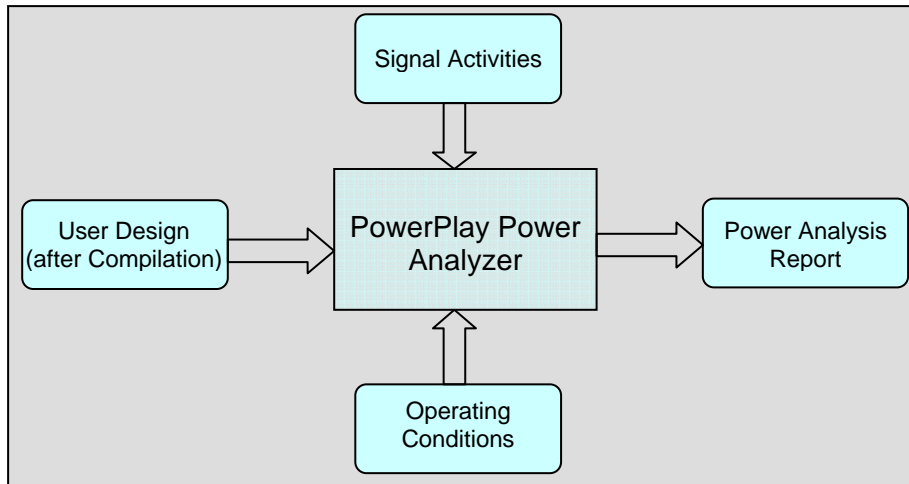
Figure 4. Quartus II PowerPlay Power Analyzer High-Level Flow
