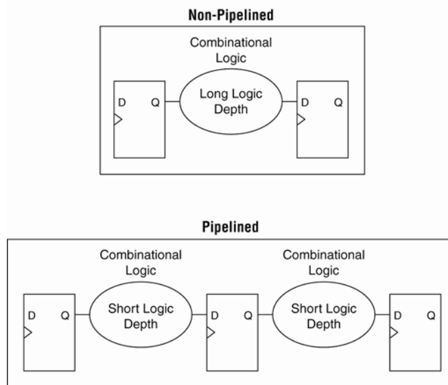
Figure 3. Pipelining Example
