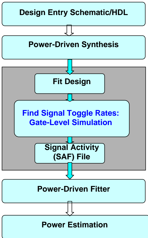
Figure 1. Quartus II Power-Driven Compilation Flow
