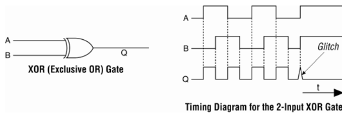
Figure 2. XOR Gate showing Glitch at the Output
