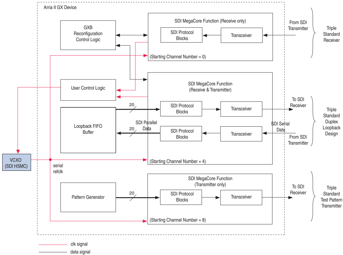
Figure 1. Block Diagram
