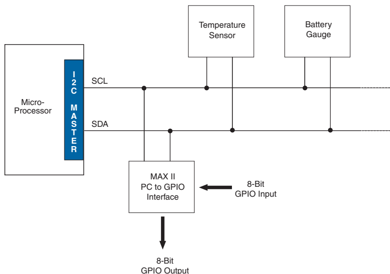
Figure 1. GPIO Pin Expansion via an I 2 C Bus
