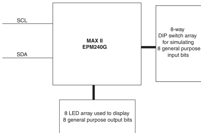
Figure 3. GPIO Pin Expansion Demonstration Circuit
