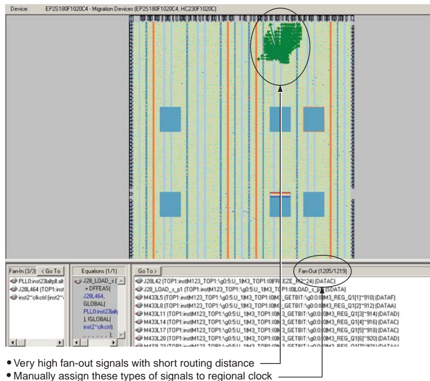
Figure 3. High Fan-Out Signals with Short Routing Distances
