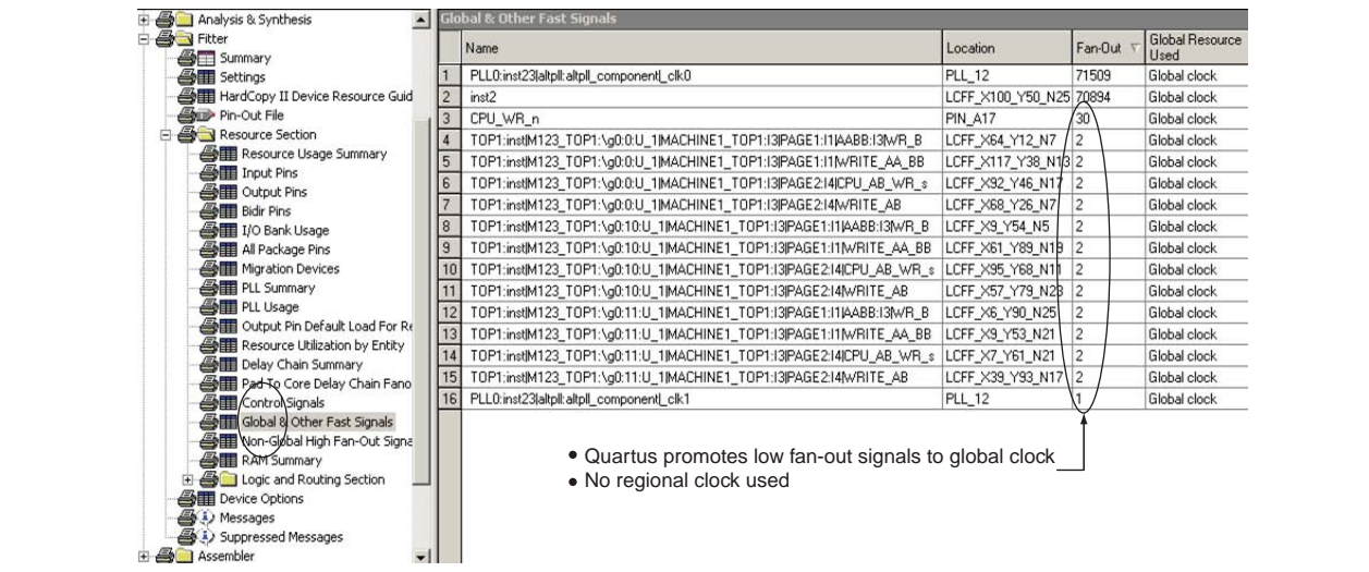
Figure 1. Example of Low Fan-Out Promotion to the Global Clock
