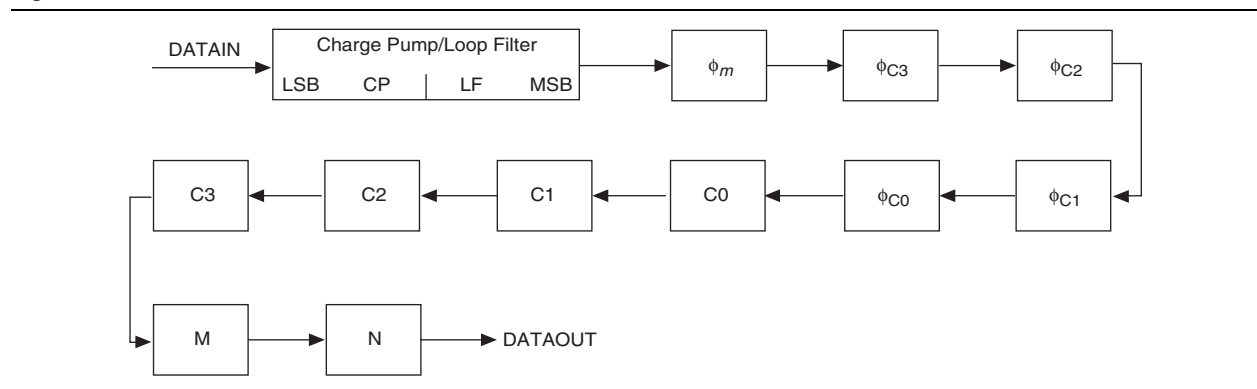
Figure 5. Scan Chain Order for Fast PLLs 1, 2, 3, 4, 7, 8, 9 and 10
