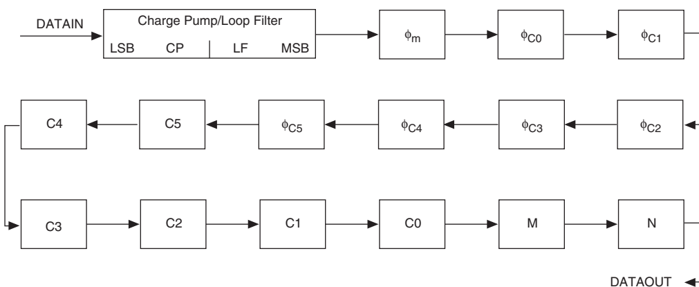
Figure 2. Scan Chain Order for Enhanced PLLs 5, 6, 11 and 12
