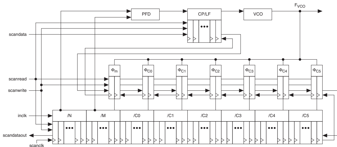
Figure 1. PLL Reconfiguration Scan Chain (Note 1)
